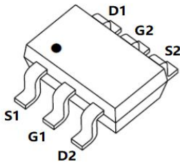
SOT-363-6L (Dual) top view
