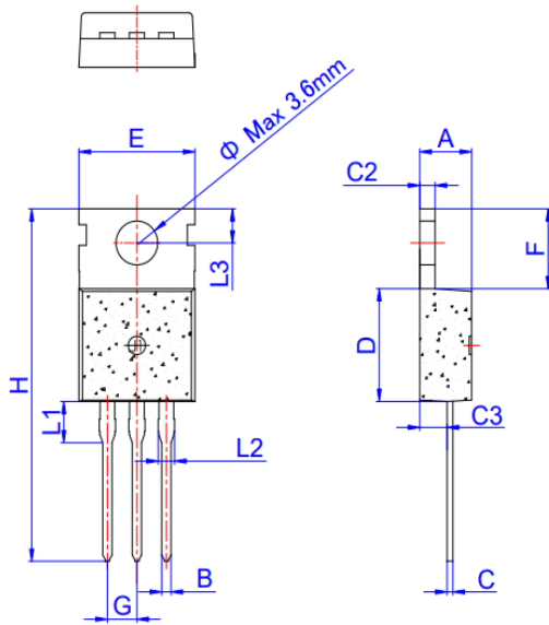
TO-220C
