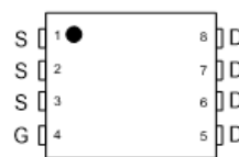
Pin Assignment
